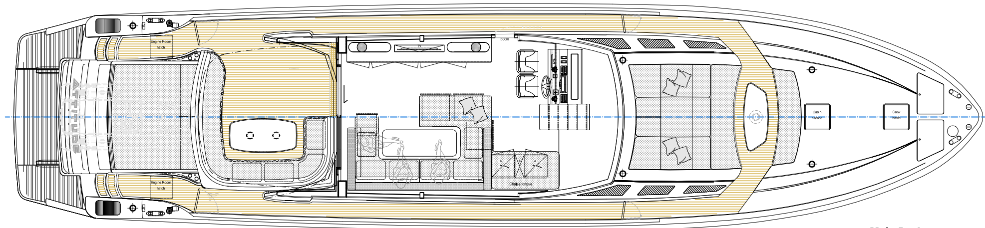
Main Deck
