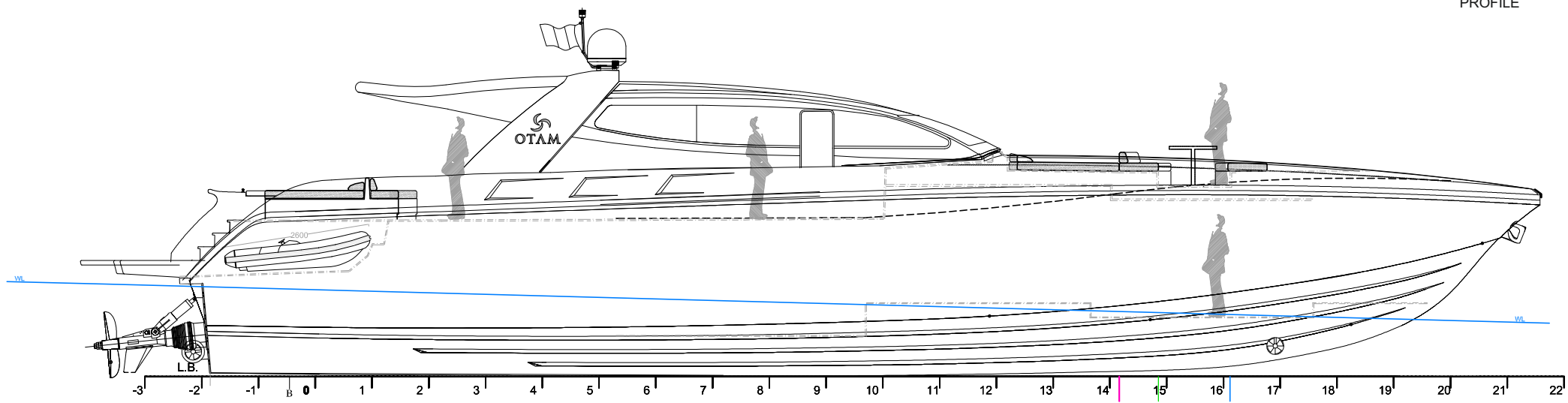
PROFILE B
